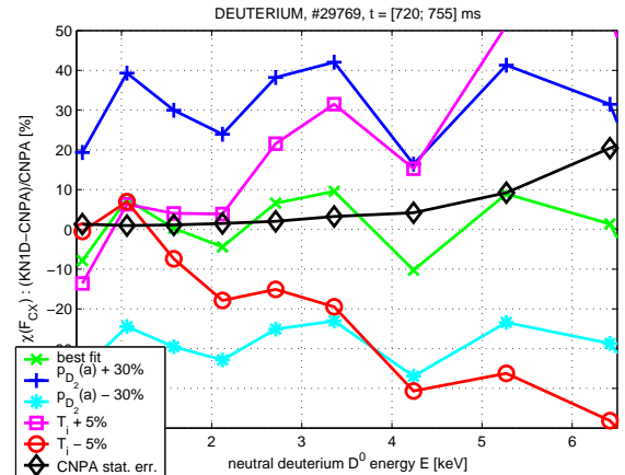
Figure 6: Relative fit error. Best fit for p_{D_2^0}(r = a) = 0.57 mTorr and T_i = T_{i,C}^{CXRS} ( \times ), p(a) \pm 30\% ( + , \bullet ) and T_i \pm 5\% ( \square , \odot )
