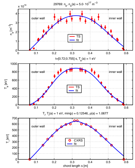
Figure 4: Plasma input profiles against CNPA chord coordinate. Diagnostics measurements ( \odot ) and fitted profiles ( \text{—} ) for n_e (top), T_e (middle) and T_i (bottom).
