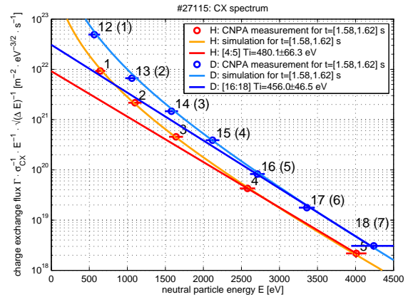
Figure 3: CNPA charge exchange spectrum with temperature fits to channels 4 & 5 and 16-18 for hydrogen and deuterium respectively.
